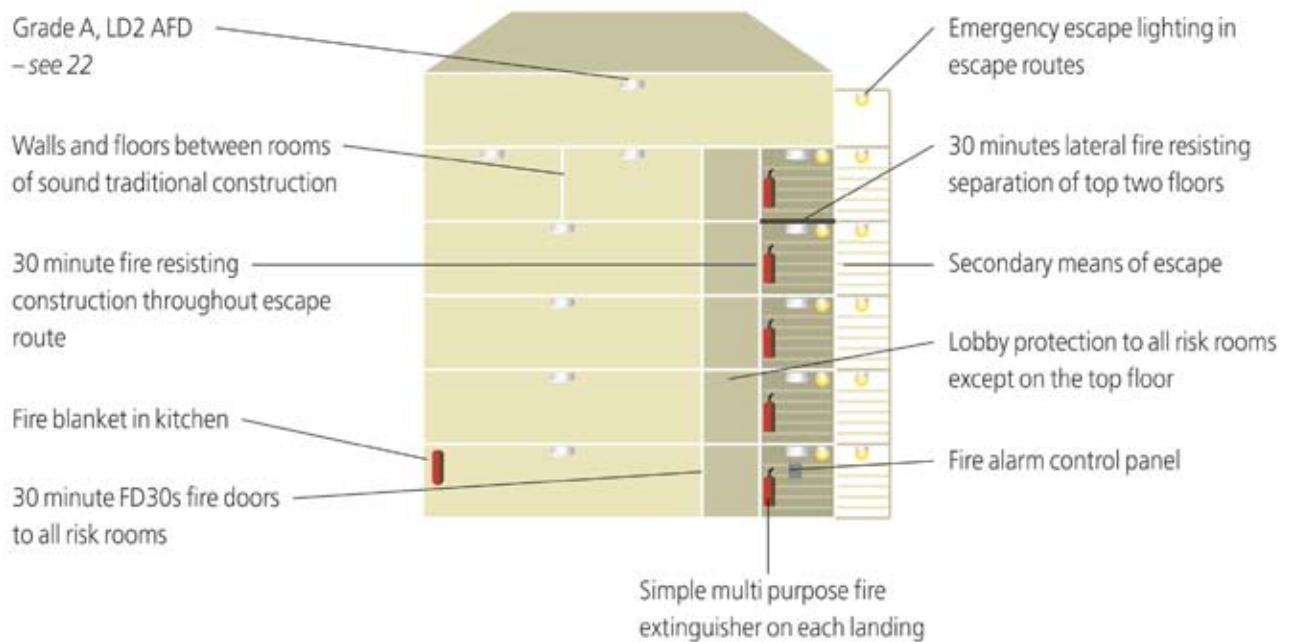
figure D6: shared house of six storeys
