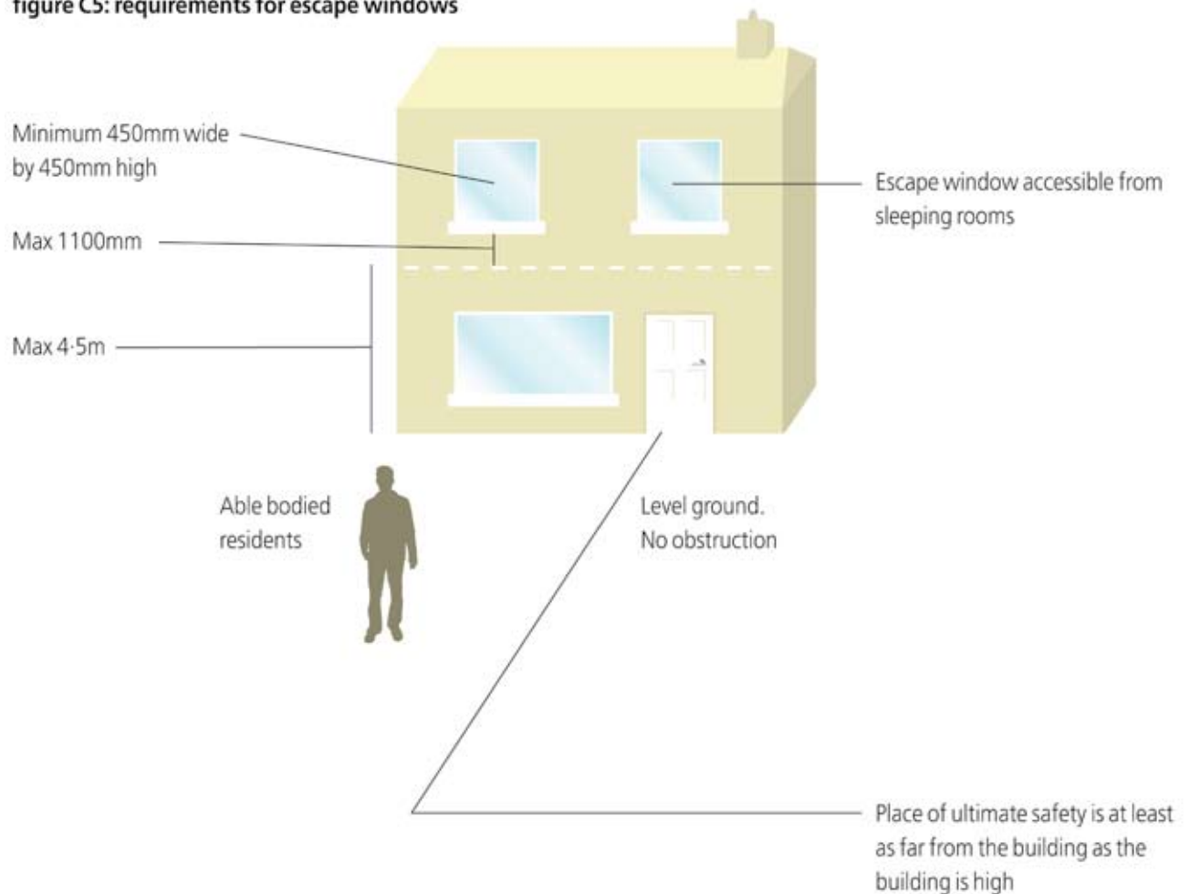
figure C5: requirements for escape windows
